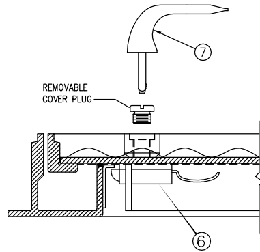
SECTION A-A STANDARD SLAM LOCK
